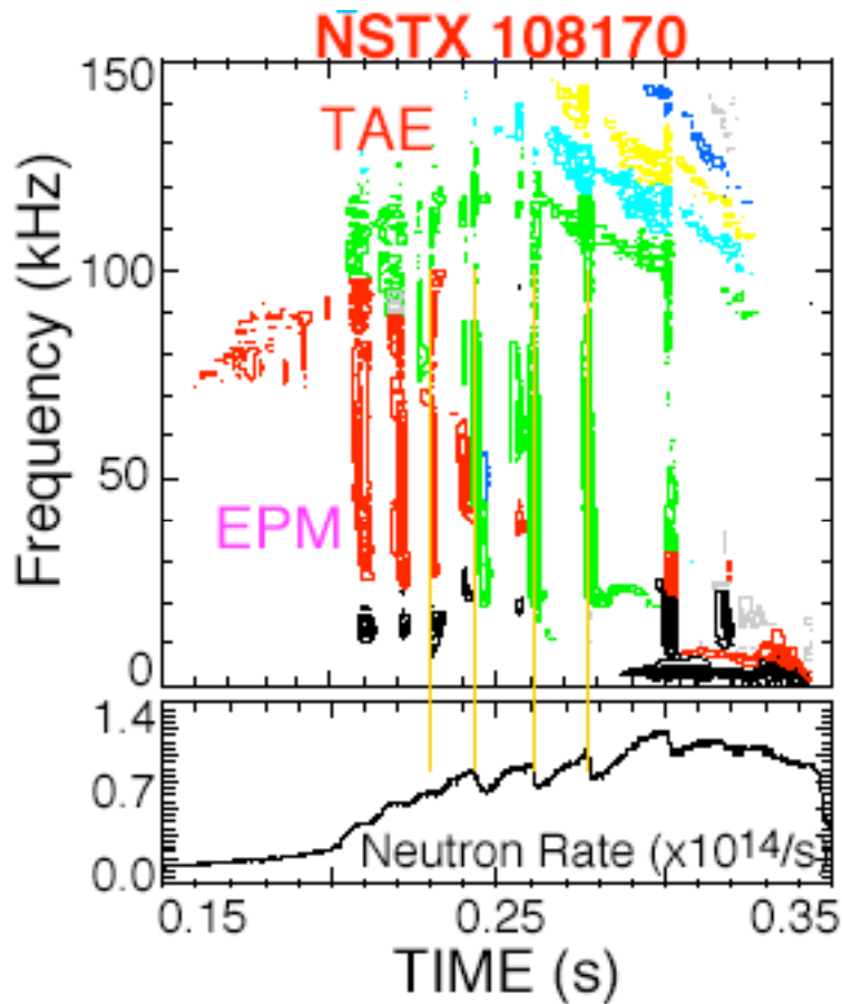
Fig. 1. A time trace of the frequency spectra of observed unstable plasma modes (TAEs and EPMS) due to the presence of super-Alfvénic high-energy ions. The bursting and chirping behavior can be seen for both TAEs and EPMS. The lower time trace shows the associated neutron drop indicative of the sudden loss of energetic ions from the reacting core.
